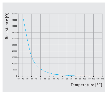
Temperature sensor characteristic curve
