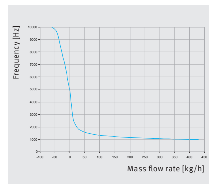
Mass flow sensor characteristic curve
